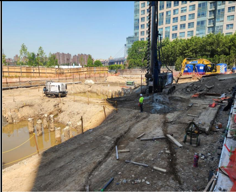
Photo 1: View of continued pile installation.
