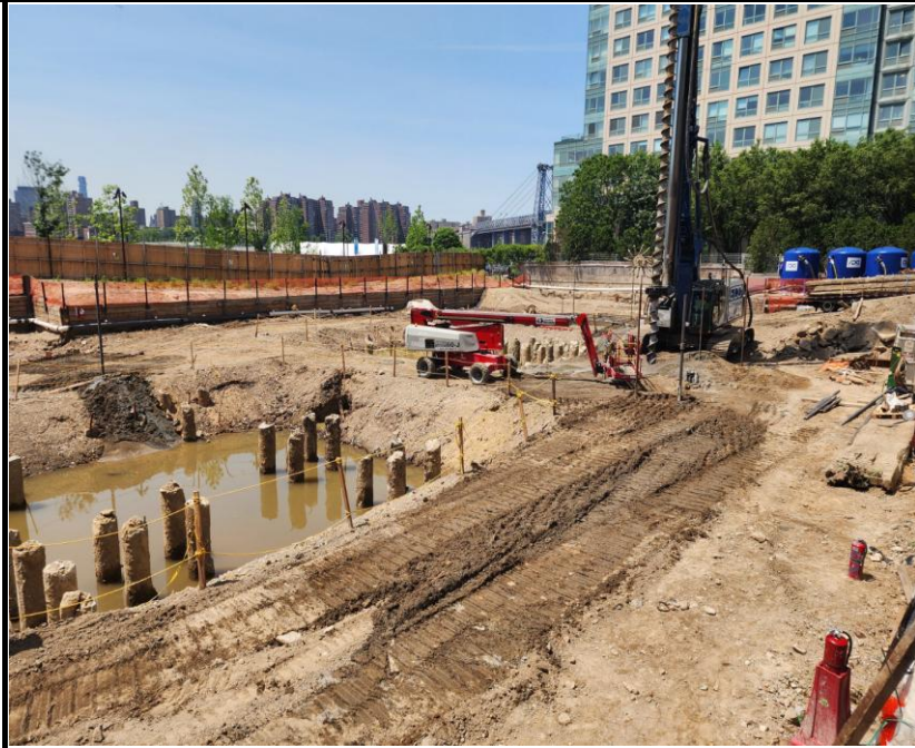
Photo 3: View of continued pile installation.
