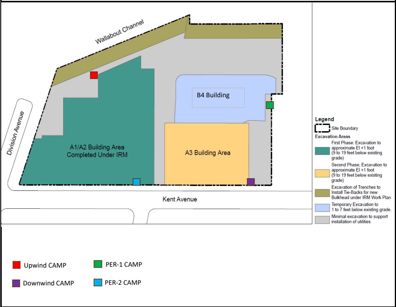
Site Layout Map and Excavation Figures
