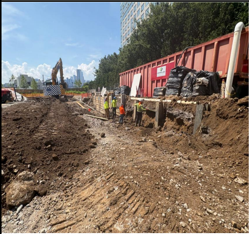
Photo 2: View of lagging installation for SOE in the utility driveway area.
