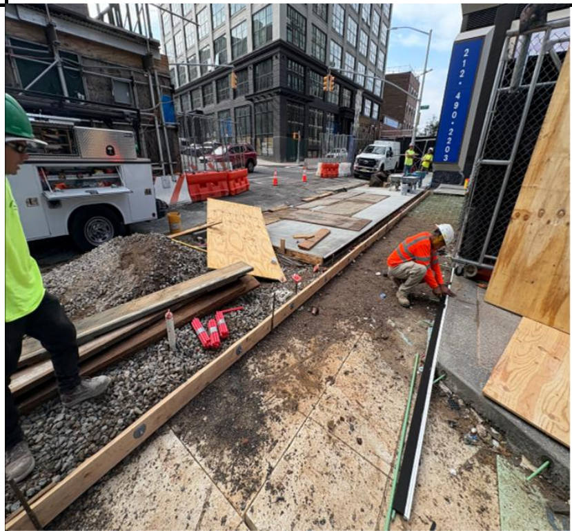
Photo 2: View of curb installation along Kent Avenue.
