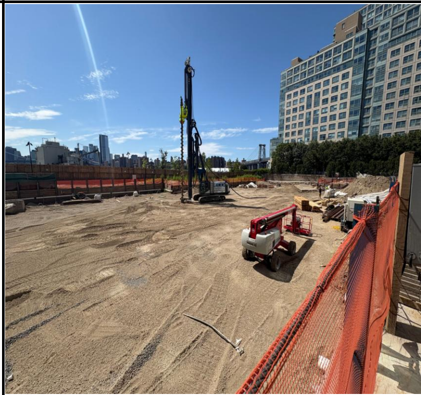
Photo 4: View of the Site conditions in the B4 footprint facing northwest.
