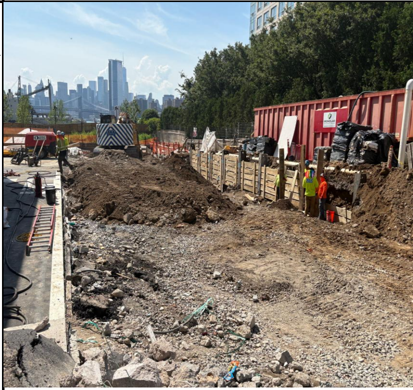
Photo 4: View of lagging installation for SOE in the utility driveway area
