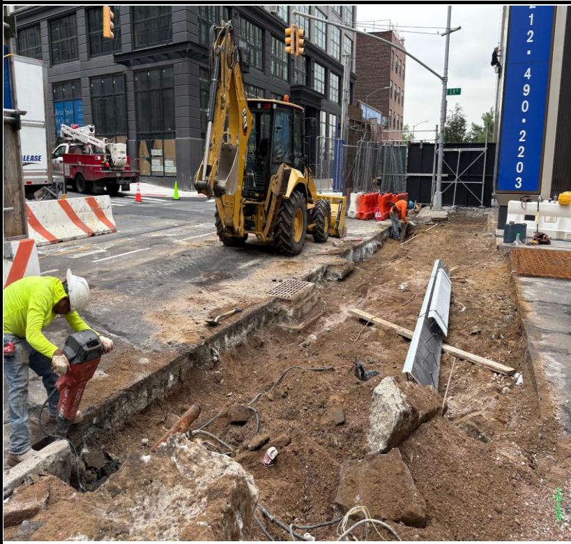
Photo 4: View of curb installation along Kent Avenue.
