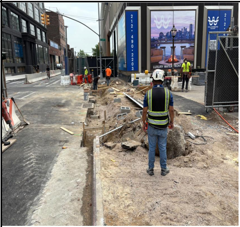
Photo 2: View of curb installation along Kent Avenue.
