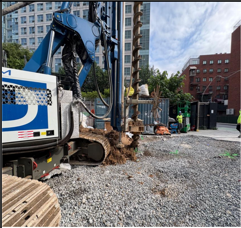
Photo 4: View of pile installation for SOE in the utility driveway area.e.
