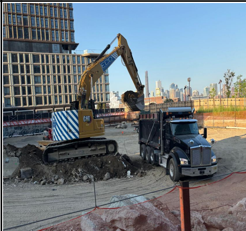
Photo 2: View of truck loading for off-site soil disposal.
