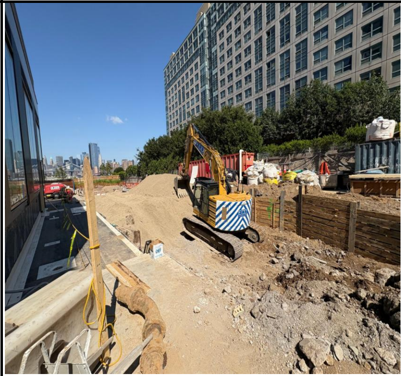
Photo 4: View of RCA cap grading.
