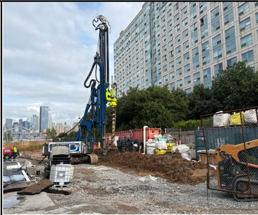
Photo 1: View of pile installation for SOE in the utility driveway area.
