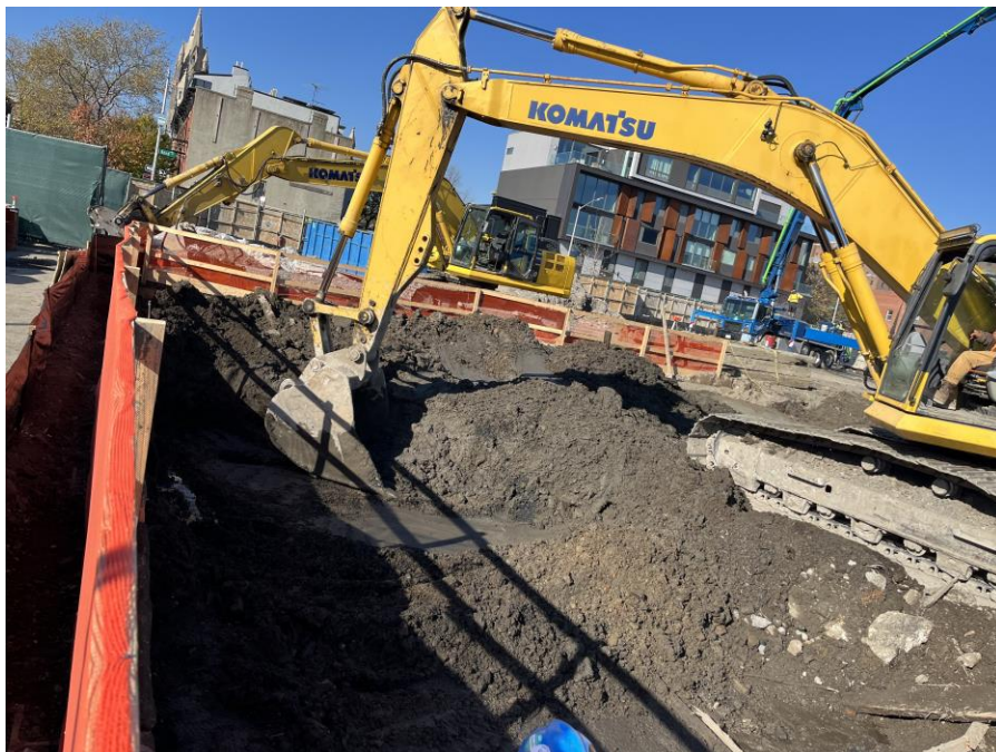
Photo 2: Kingdom excavating to install lagging in the southern part of Society Brooklyn (facing west)
