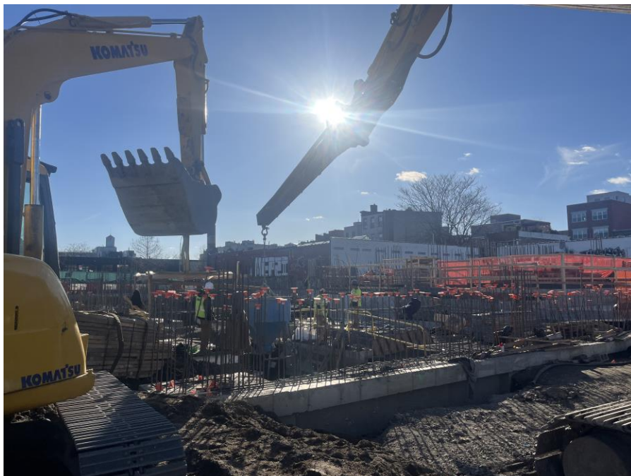
Photo 2: Kingdom placing concrete for structural pile caps in the northern part of Sackett Place (facing east)
