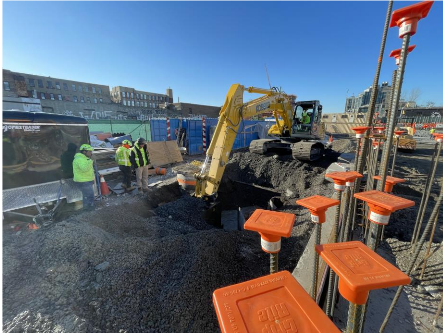
Photo 1: G&M installing utilities in the eastern part of Sackett Place within the SPW (facing southeast)
