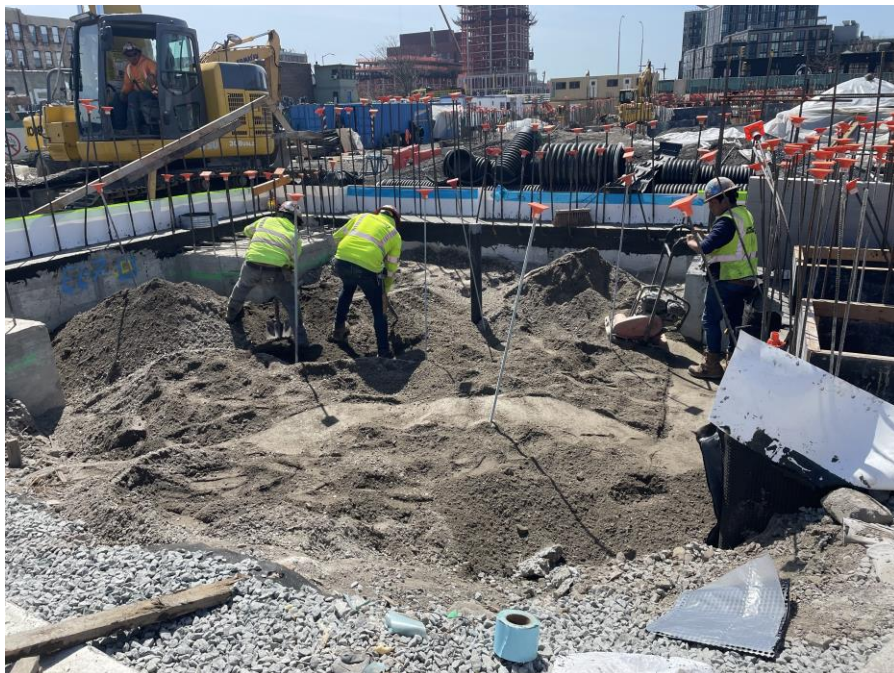
Photo 2: Kingdom backfilling around utilities in the southern part of Society Brooklyn (facing south)
