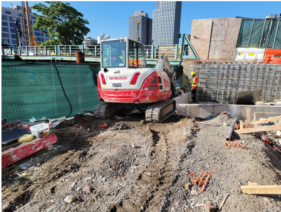
Photo 2: G&M excavating to install foundation elements in the southern part of Sackett Place within the SPW (facing south)
