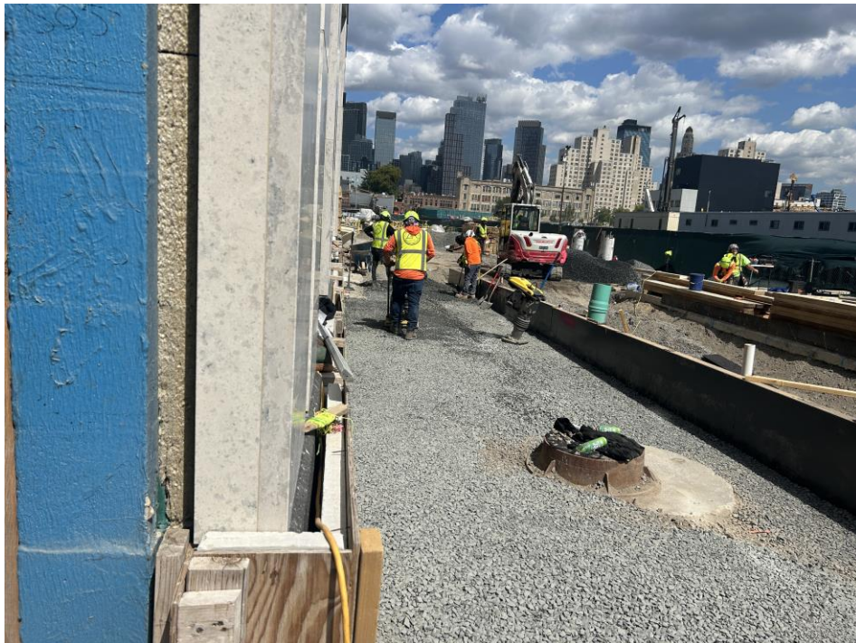
Photo 2: G&M backfilling in the southern part of the SPW (facing north)
