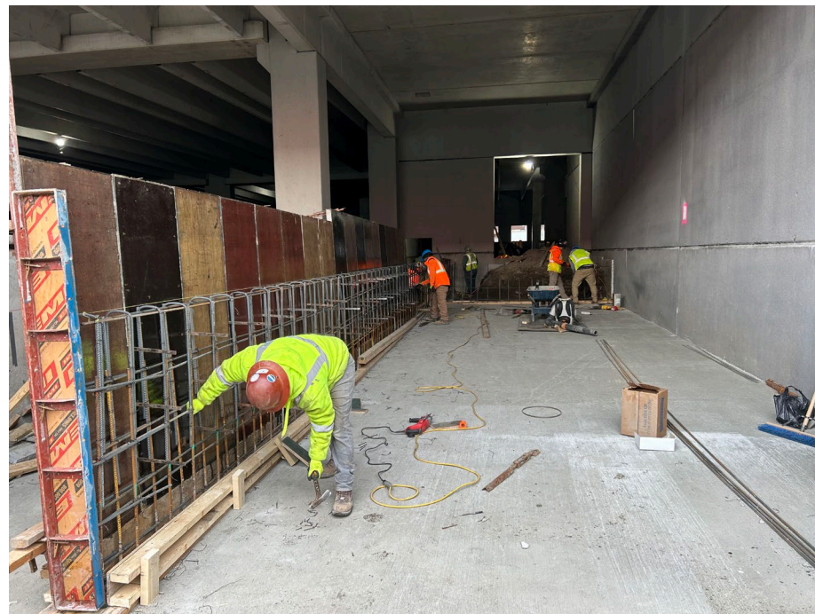
Photo 4: Forms and rebar placed to pour half-walls in grid B3.
