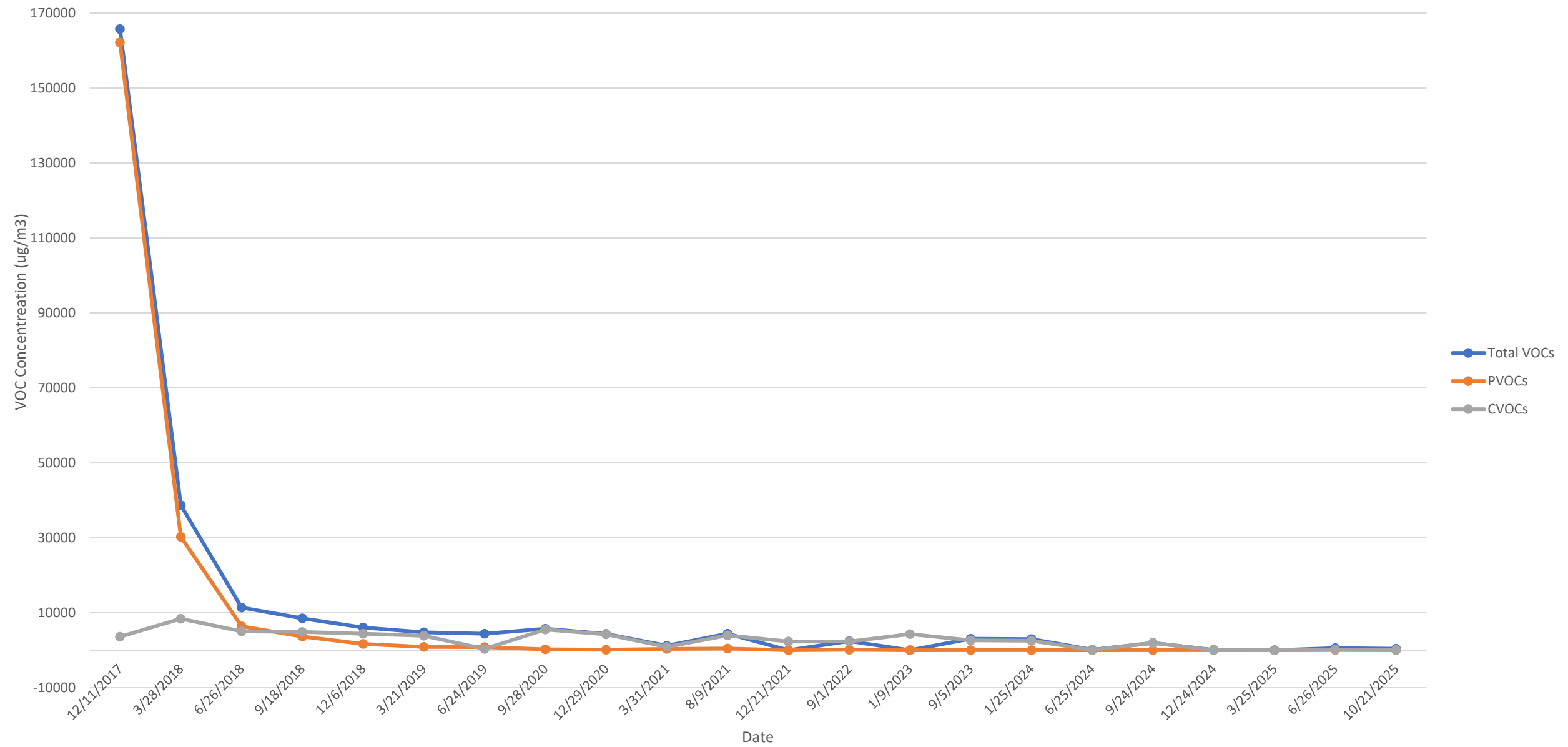
Graph 5 SVE System Influent 1103-1107 Dekalb Avenue, Brooklyn, NY October 2017- October 2025
