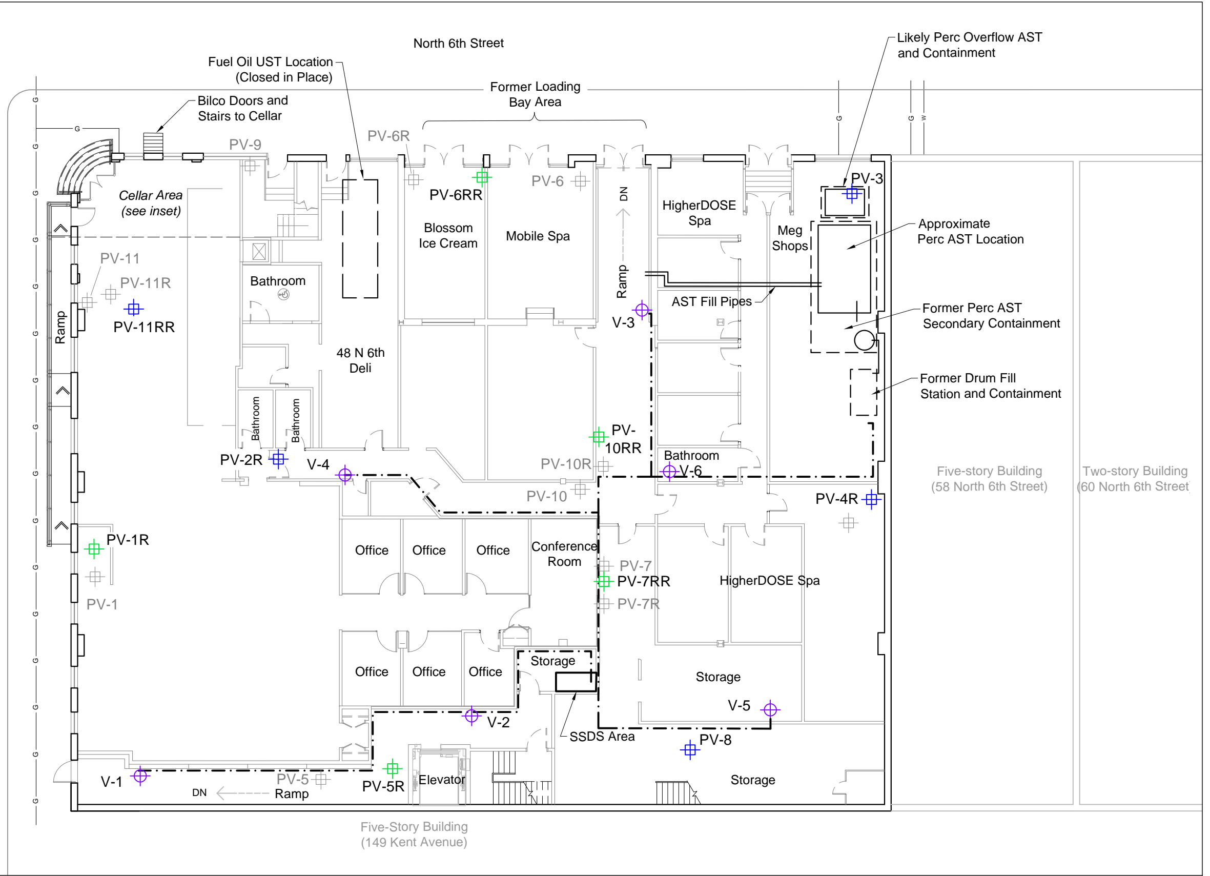
Figure 1. Site Sub-Slab Depressurization System and Monitoring Points 135 Kent Avenue, Brooklyn, NY
