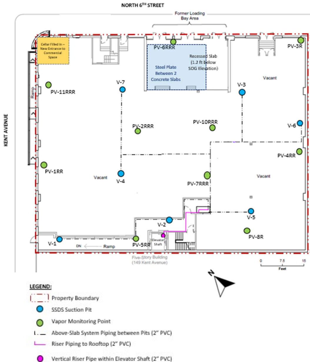
Figure 1 – First Floor SSDS Layout
