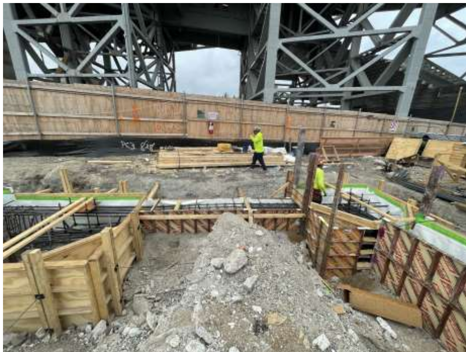
Photo 2: Bauer installing waterproofing/vapor barrier along the exterior foundation walls prior to concrete pour (facing south).
