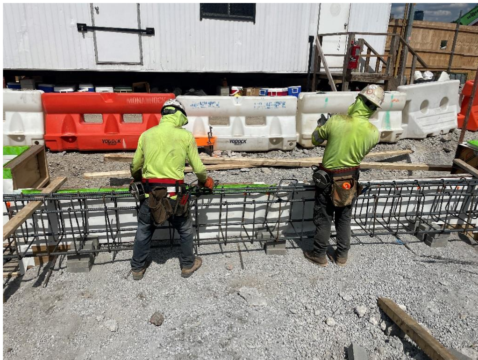
Photo 2: Bauer installing formwork in the northern part of the site (facing north)
