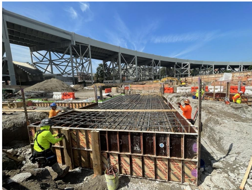
Photo 2: Bauer installing formwork in the north-central part of the site (facing west).
