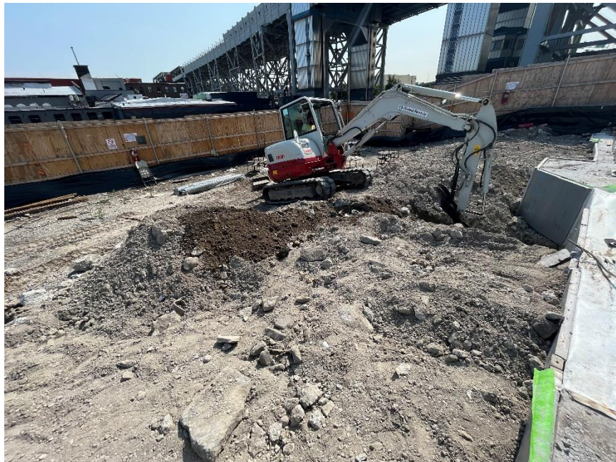
Photo 2: Bauer excavating in the southeastern part of the site for the continued installation of a storm drain (facing southeast).
