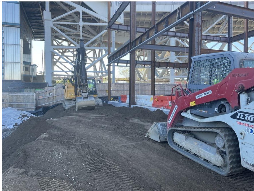
Photo 2: Bauer grading the backfill area in the southeastern part of the site (facing south)
