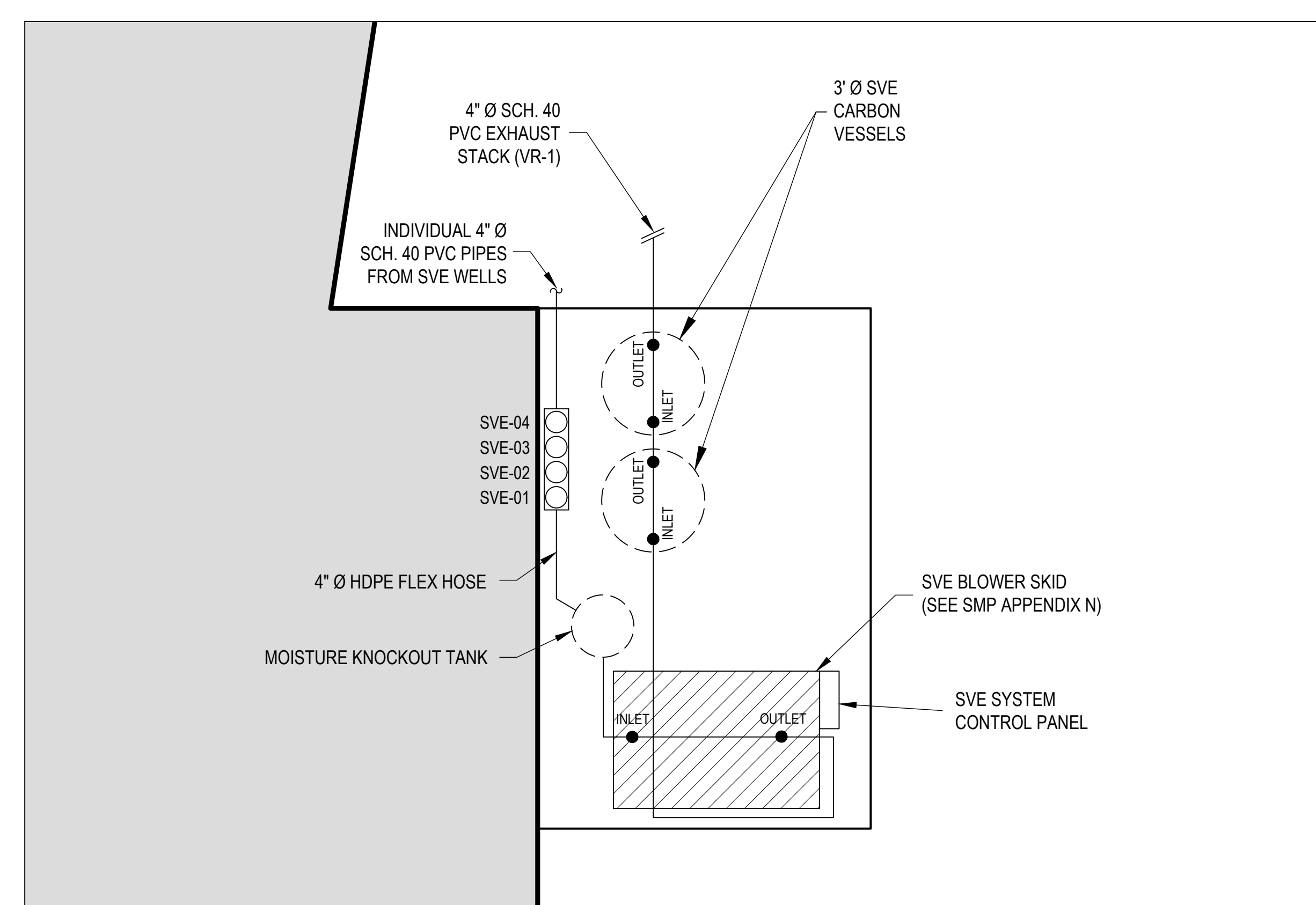
2 SVE EQUIPMENT AREA FIG 3
