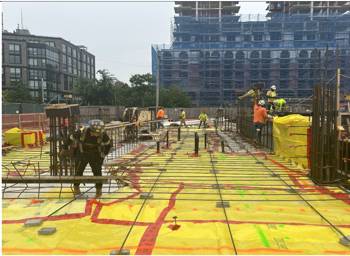
Photo 1 – Representative photo of vapor barrier and rebar installation in the south building.
