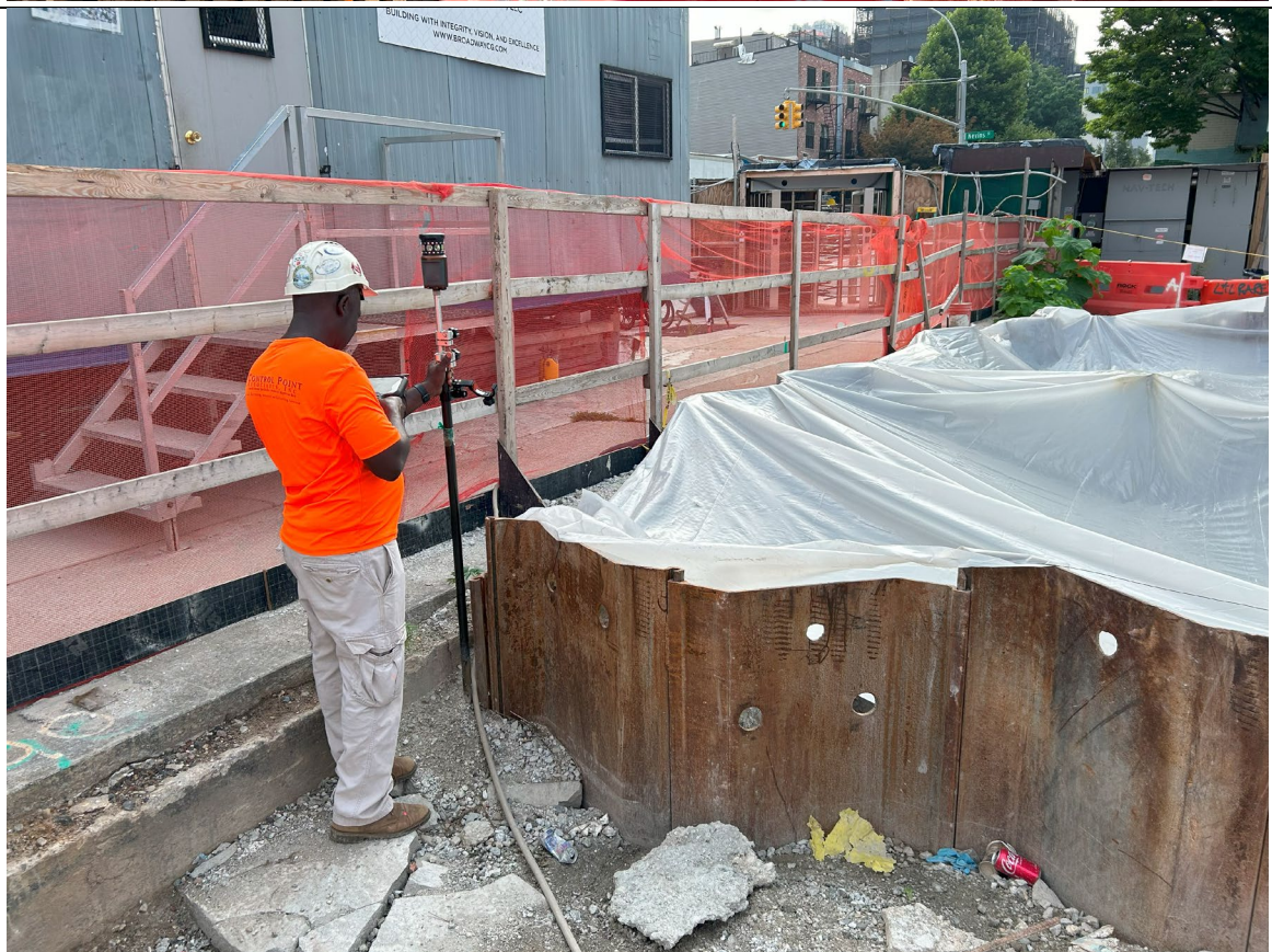
Photo 4 – Representative photo of Control Point surveying along Spill 2308807 sheeting.
