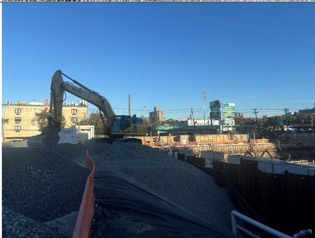
Photo 4 – United backfilling in the northeastern portion of the Site with 1.5-inch stone, facing north.
