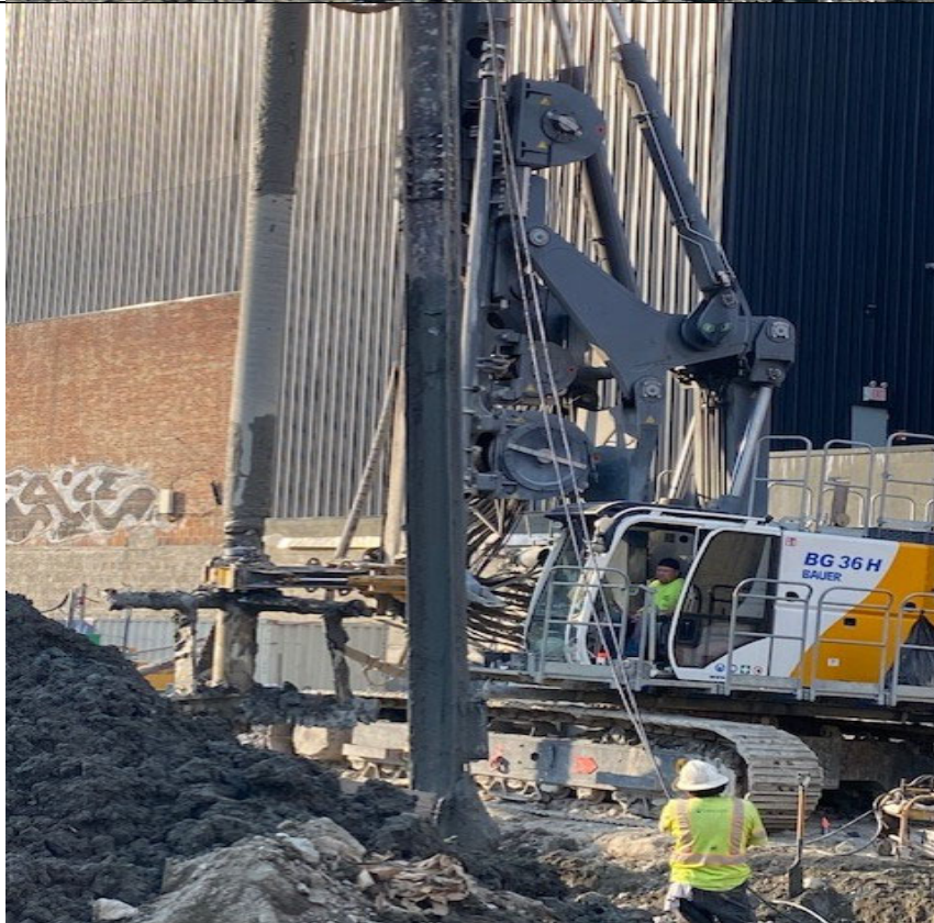
Photo 2- Representative photo of bar used to collect wet-mix sample from completed column.
