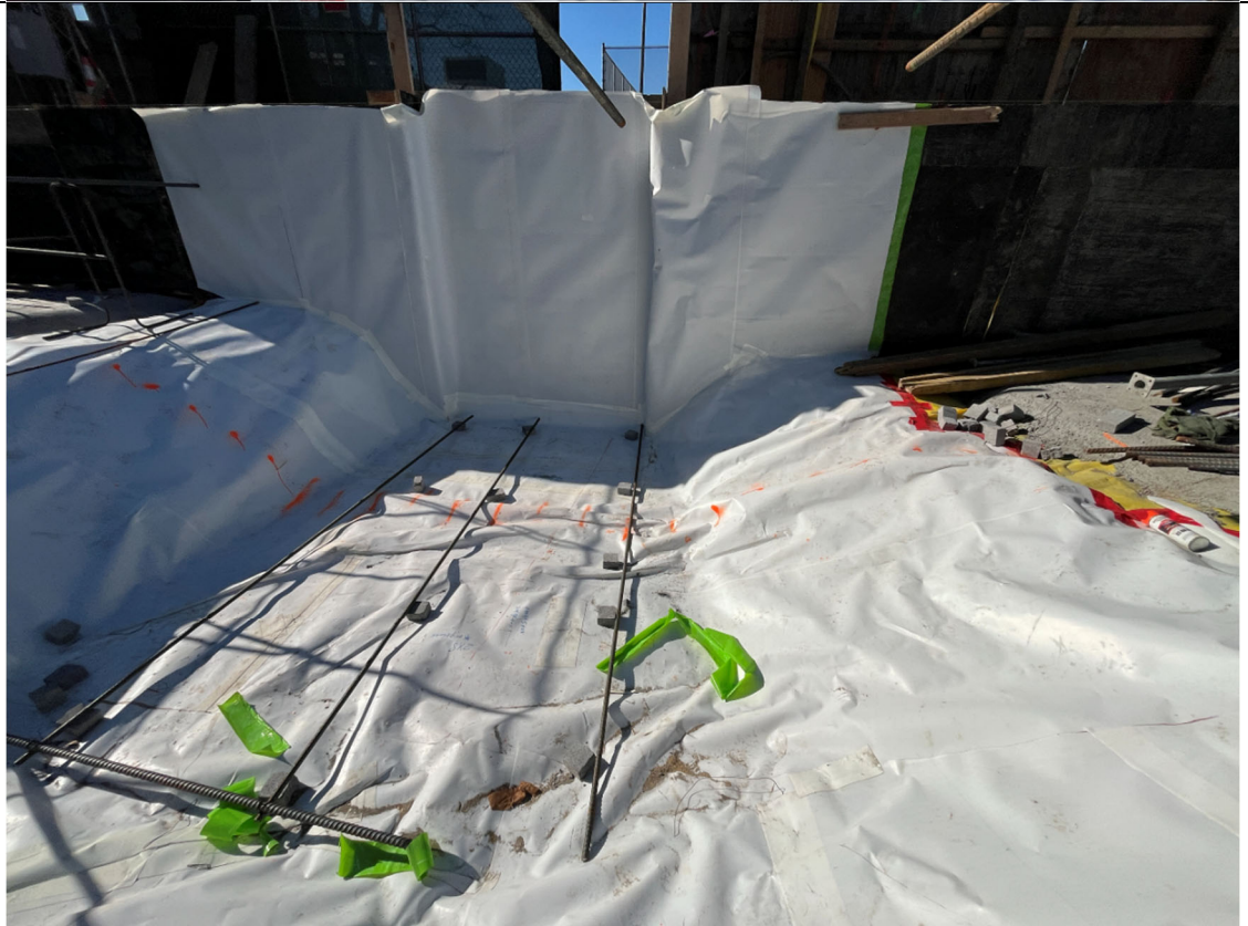
Photo 4- Representative photo of waterproofing adjacent to Douglass Street.
