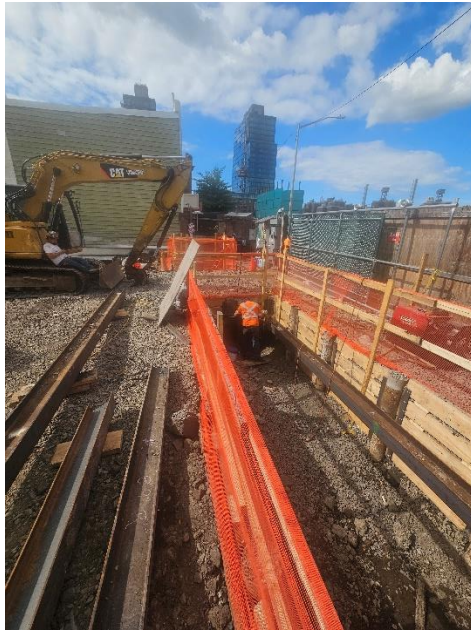
Photo 1: View of contractor welding I beams in the northeastern area of the Site, facing West.
