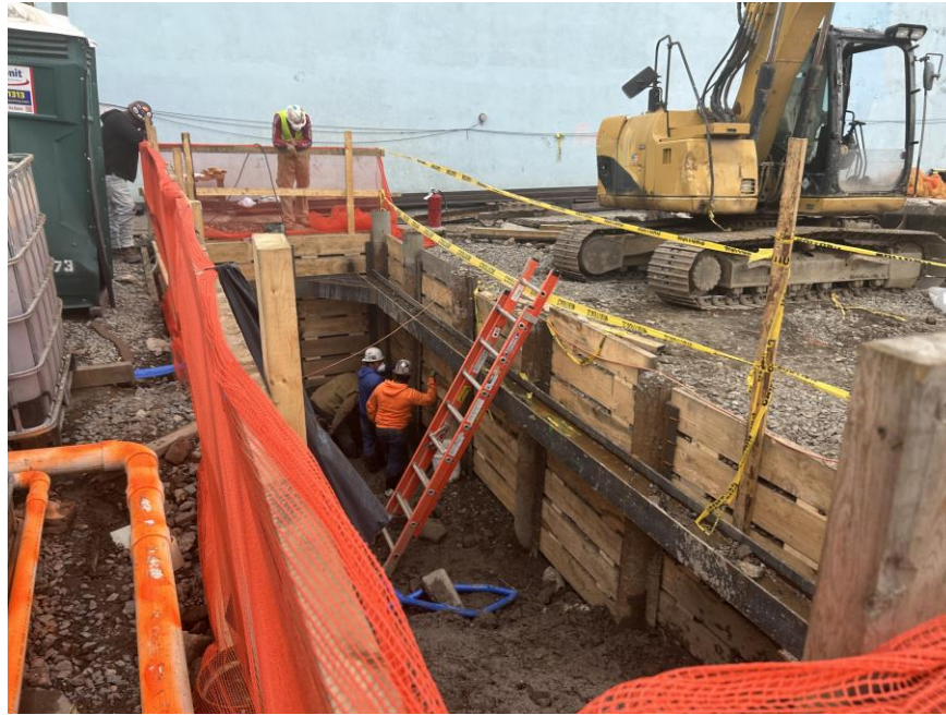
Photo 1: View of contractor Installing SOE, facing East.
