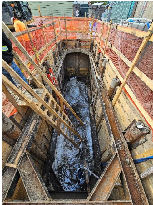
Photo 2: View of northern excavation with odor suppressant foam and poly sheeting covering, facing West.
