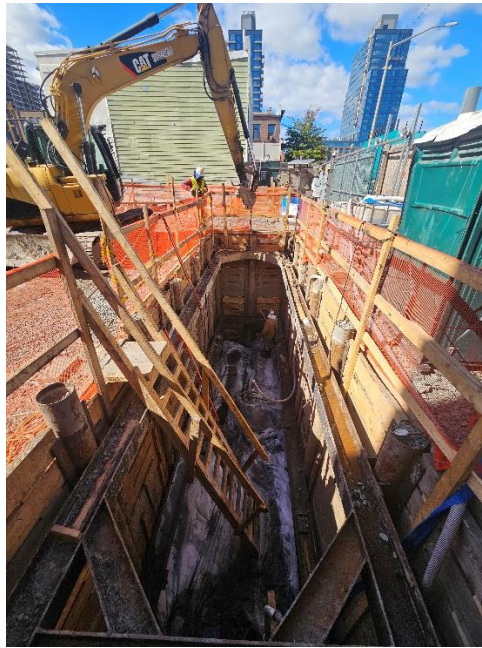
Photo 1: View of contractor installing waler beams, facing West.
