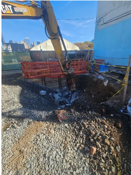
Photo 1: View of contractor chipping concrete footing for removal, facing North.
