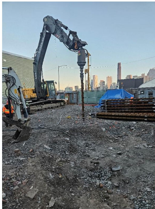
Photo 2: View of Blanco installing structural pile, facing Northwest.
