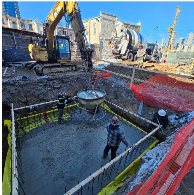
Photo 2: View of contractor pouring concrete for water tank base, facing Northwest.
