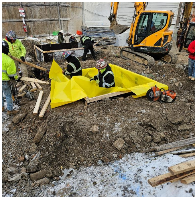
Photo 2: View of contractor installing vapor barrier in footing forms, facing West.
