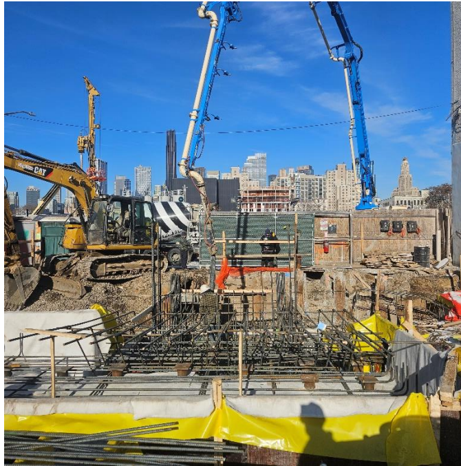
Photo 1: View of contractor pouring concrete for footings, facing North.
