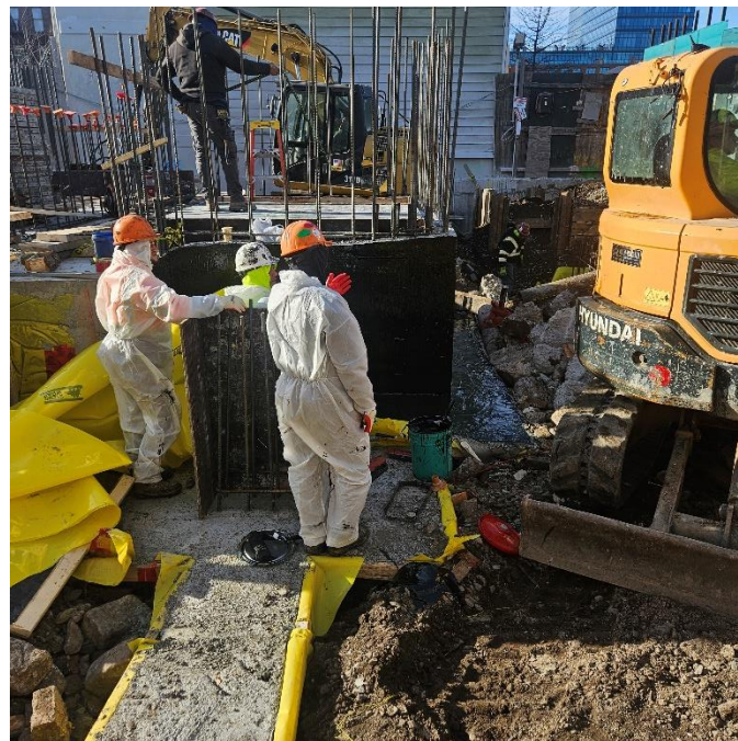
Photo 2: View of contractor installing waterproofing on central footing, facing West.
