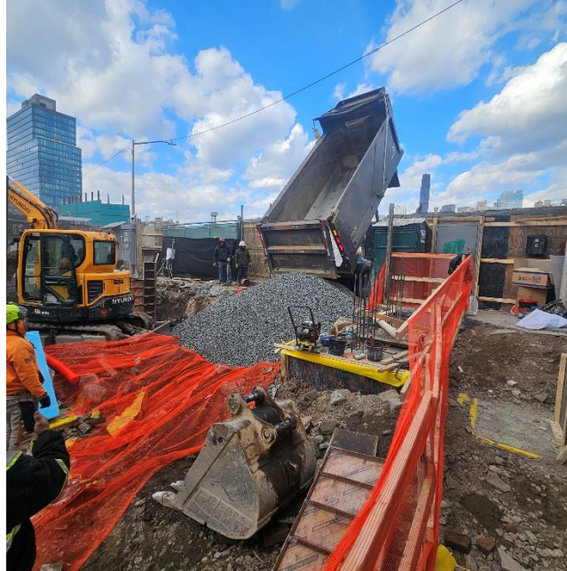
Photo 1: View of contractor unloading ¾ in stone for backfill, facing North.
