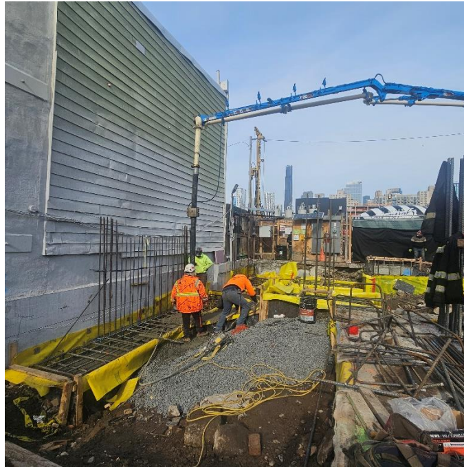
Photo 1: View of contractor pouring concrete for footings, facing Northwest.
