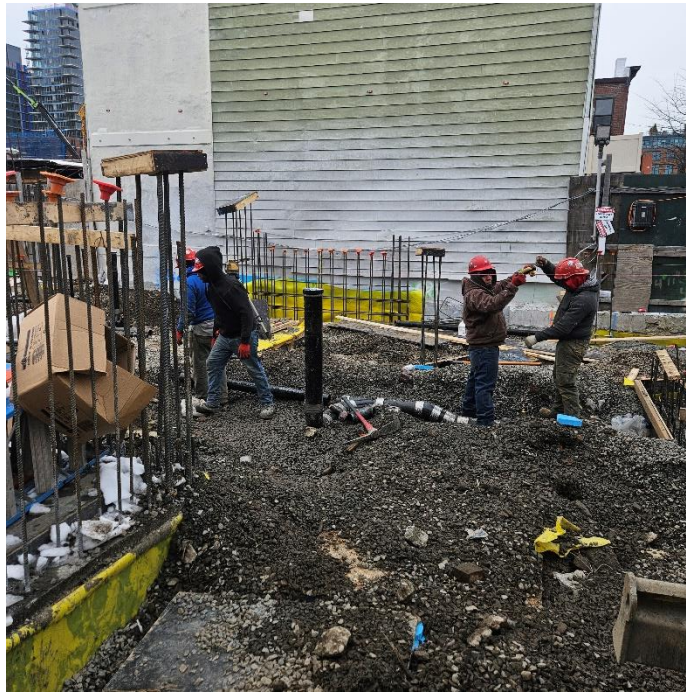
Photo 1: View of contractor installing plumbing elements, facing West.
