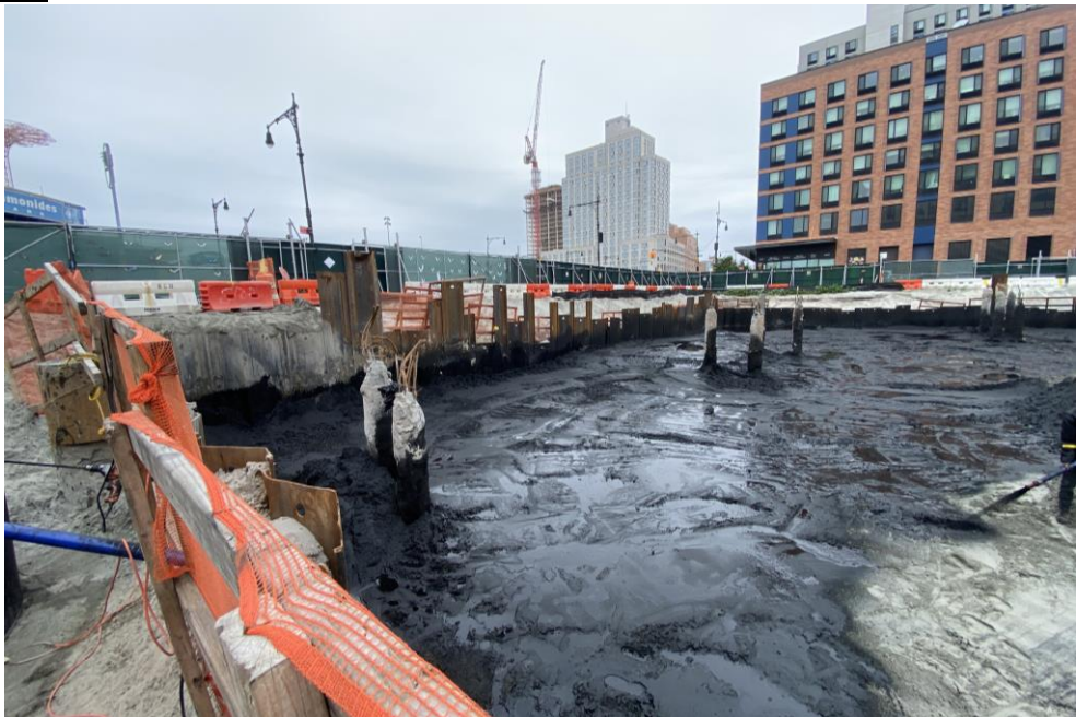
Photo 1: View of the remedial product applied within the excavation in the southern part of the site (facing southwest).
