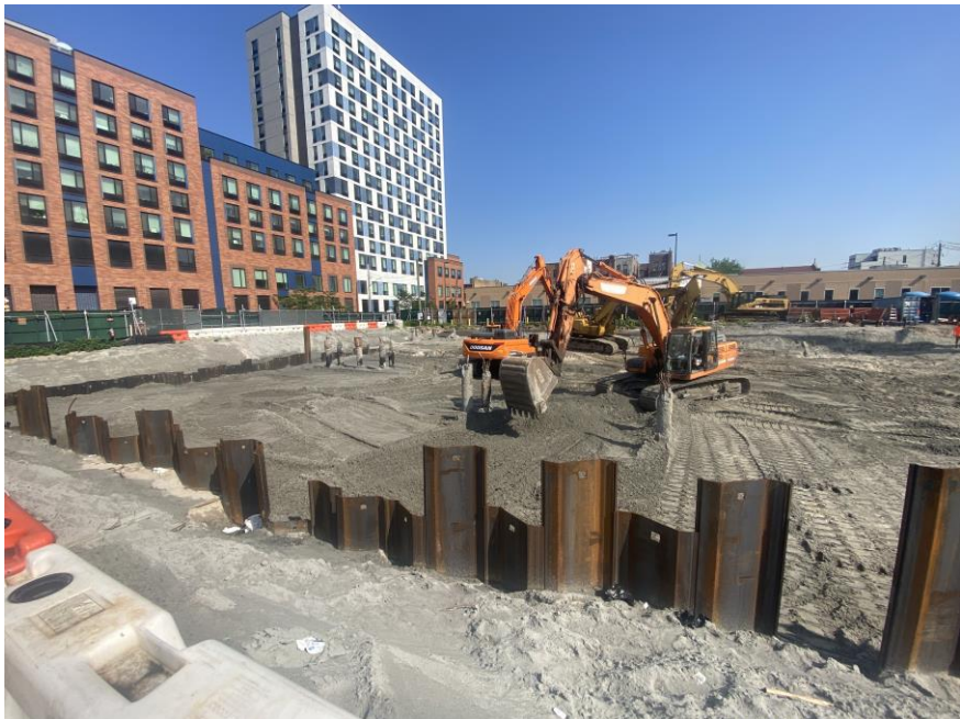
Photo 2: Precise grading pipe sand in the southern part of the site (facing northwest).
