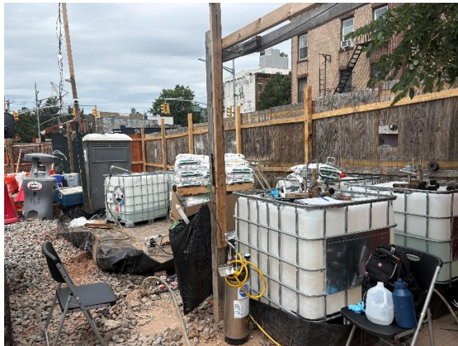
Photo 2: View of Isotec performing ISCO injections pilot test at IW-9, facing north.
