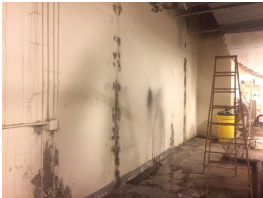
Photo 10: Surface cover and wall grout injections in Site boiler room.
