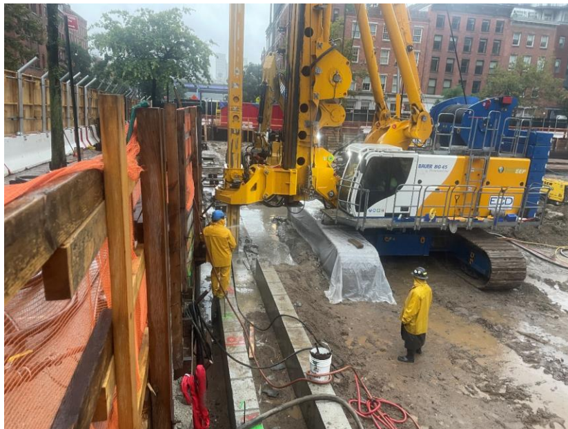
Photo 2: ECD installing a soil mix column in the eastern part of the site (facing south)
