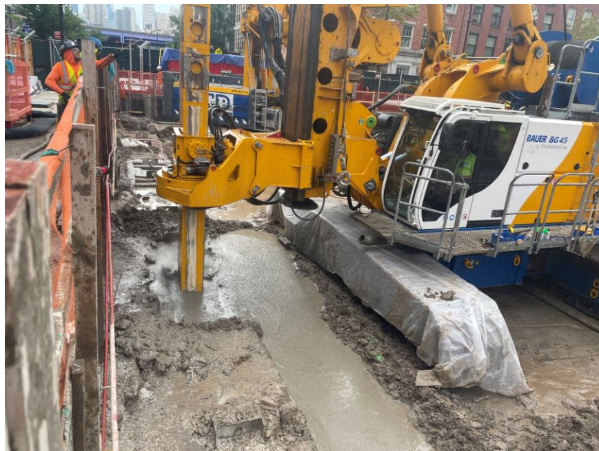
Photo 2: ECD installing a soil mix column in the eastern part of the site (facing southeast)
