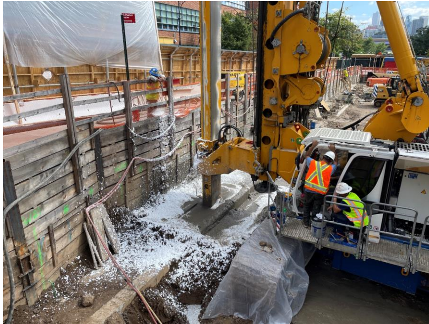
Photo 1: Atmos® AC-645 odor/vapor suppressing foam applied during soil mix column installation in the eastern part of the site (facing southeast)
