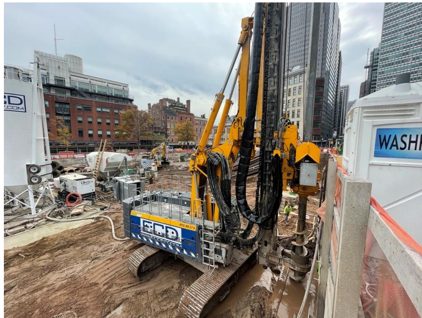
Photo 2: ECD pre-drilling a borehole in northern part of the site in preparation for soil mix column installation (facing southwest)
