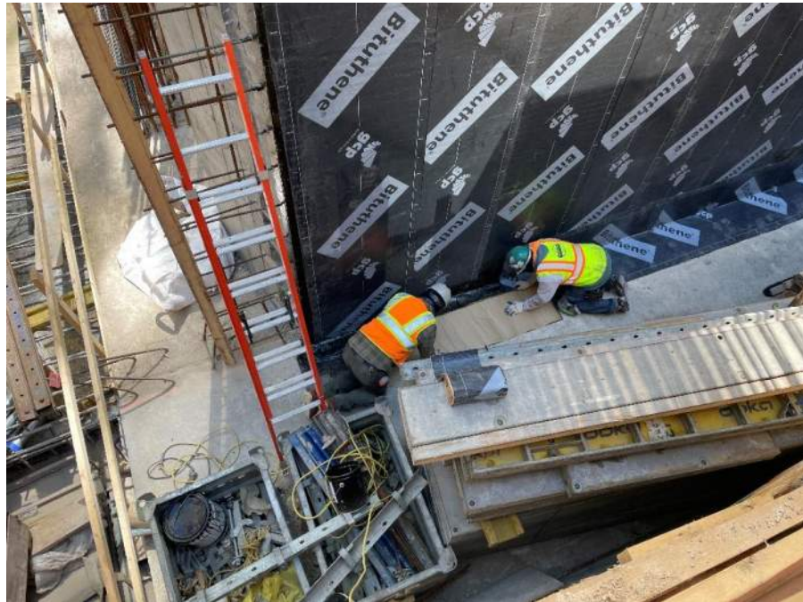
Photo 1: View of Urban installing waterproofing/vapor barrier membranes within the central part of the site (facing north).
