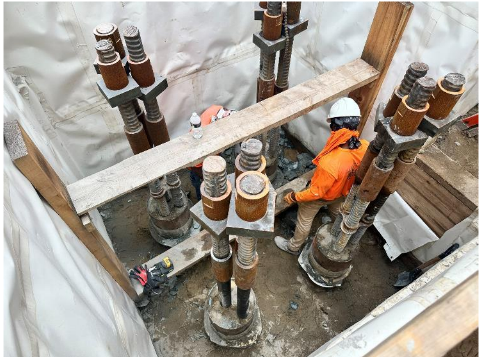
Photo 2: View of Urban removing concrete in the southern part of the site (facing northeast).
