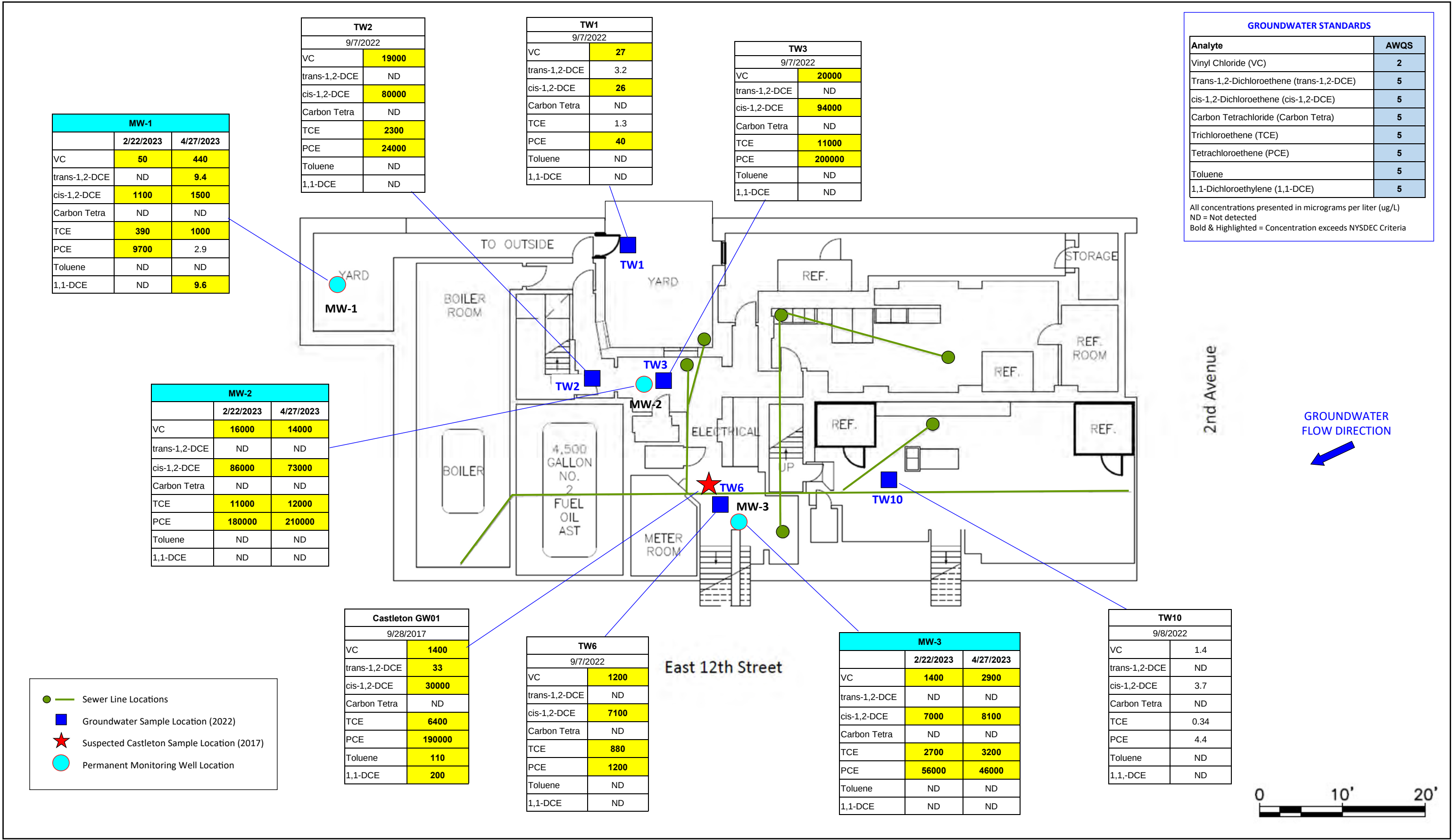
GROUNDWATER SAMPLE RESULTS MAP 300 EAST 12th STREET NEW YORK, NEW YORK
