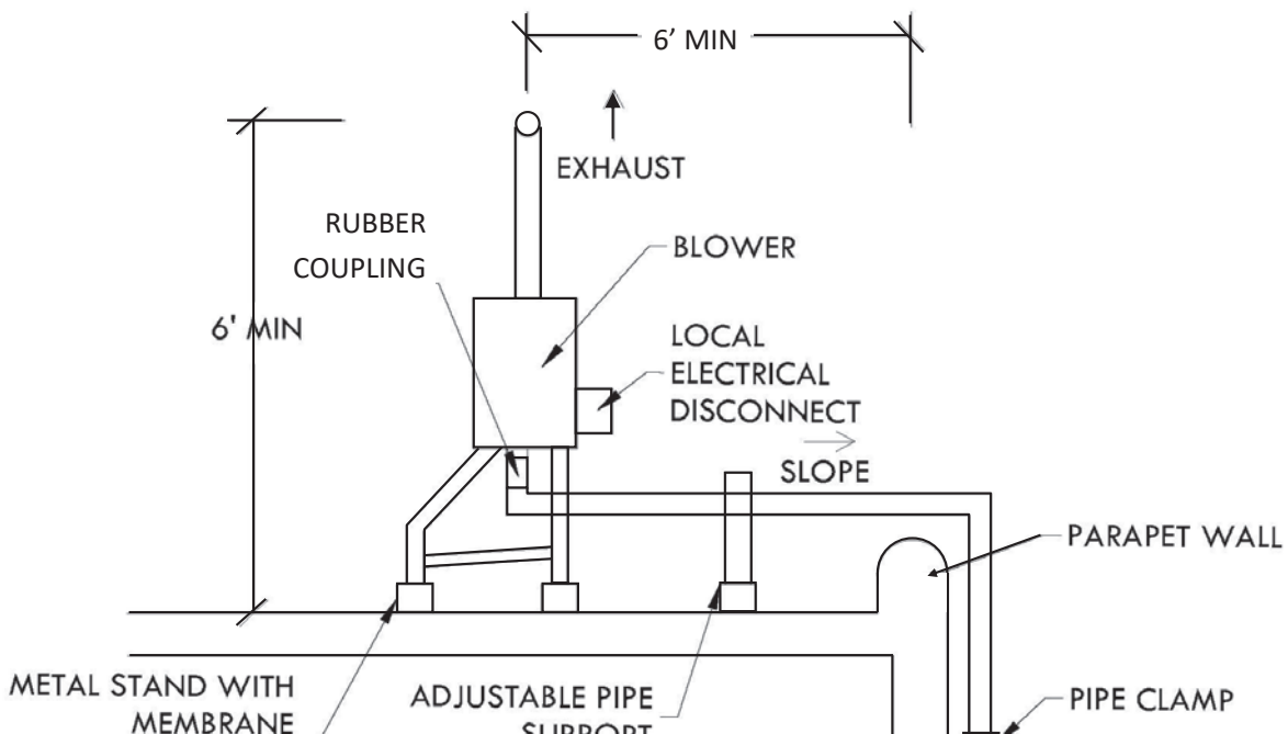
FAN MOUNT DETAIL SCALE: NOT TO SCALE
