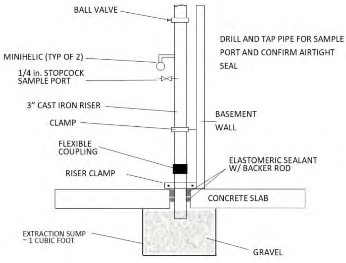
VERTICAL EXTRACTION RISER DETAIL w/SUMP SCALE: NOT TO SCALE
