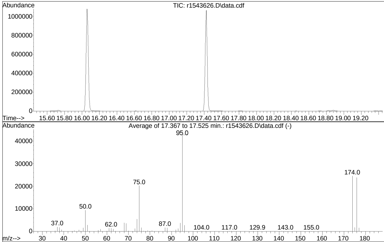
Spectrum Information: Average of 17.367 to 17.525 min.
