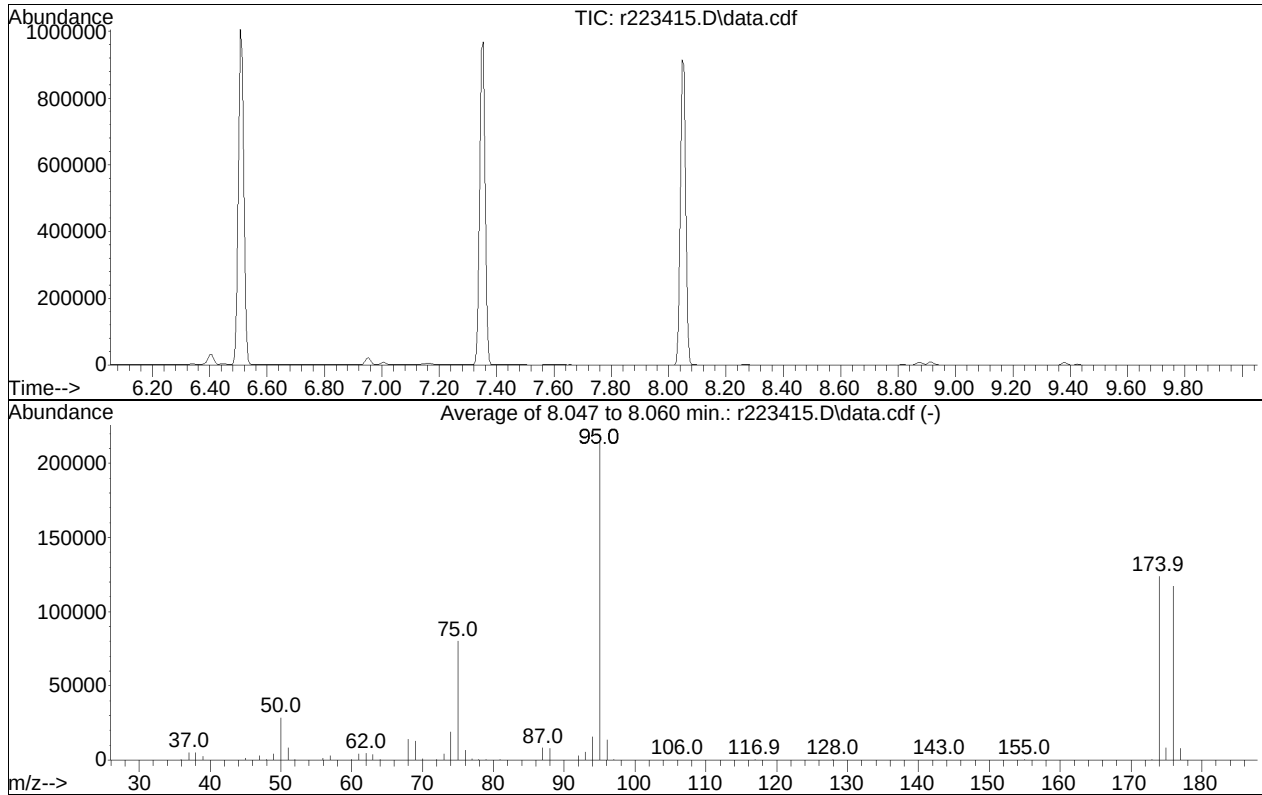
Spectrum Information: Average of 8.047 to 8.060 min.
