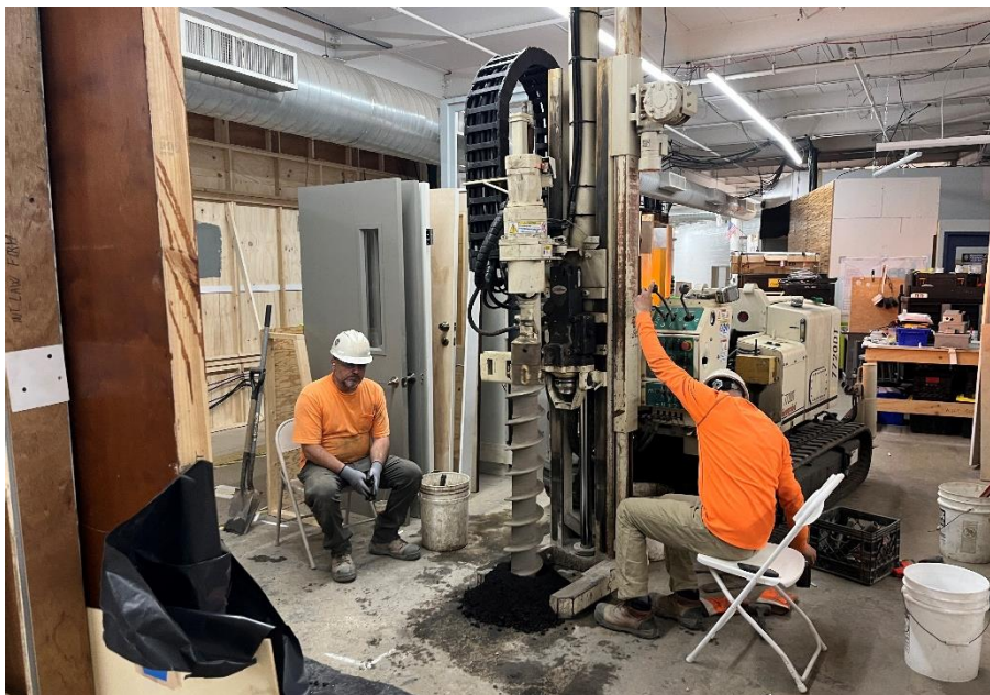
Photo 2: Geoprobe 7720DT augering monitoring well MW-4
