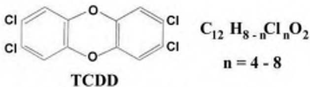
2,3,7,8-tetrachloro-dibenzo-p-dioxin
