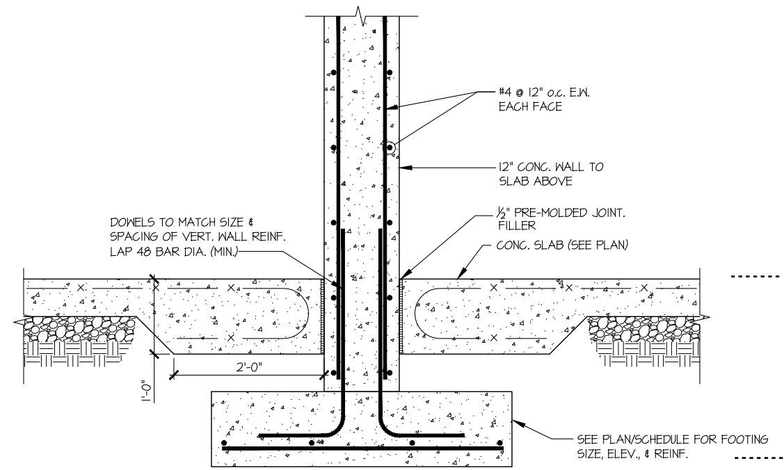
2 SECTION @ 12" INTERIOR WALL SCALE: 3/4"=1'-0"
