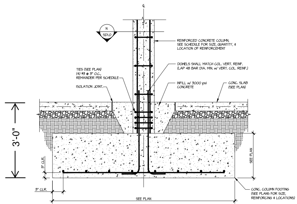
1 SECTION @ COL. FOOTING SCALE: 3/4"=1'-0"
